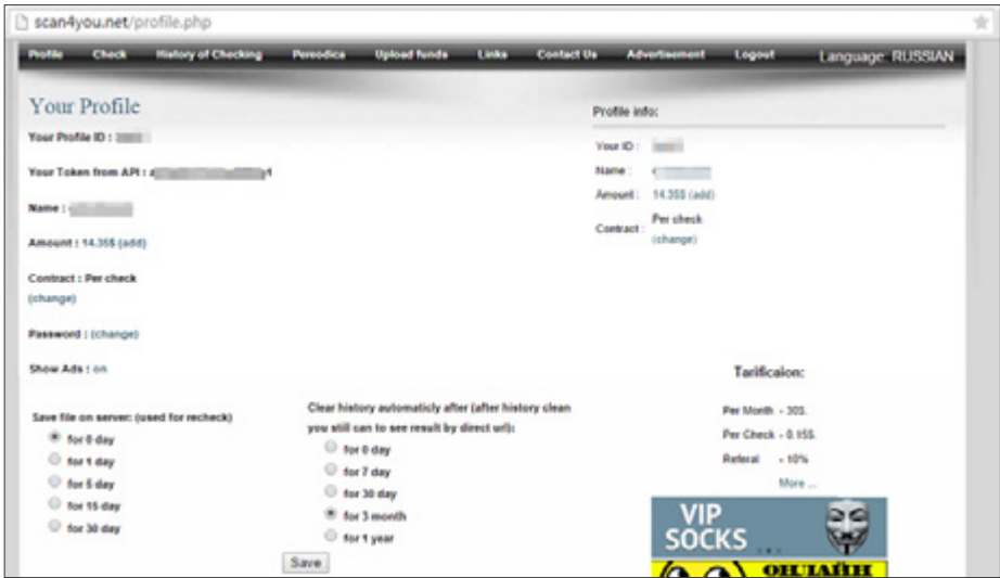
Screenshot of Uche’s profile in Scan4You.
